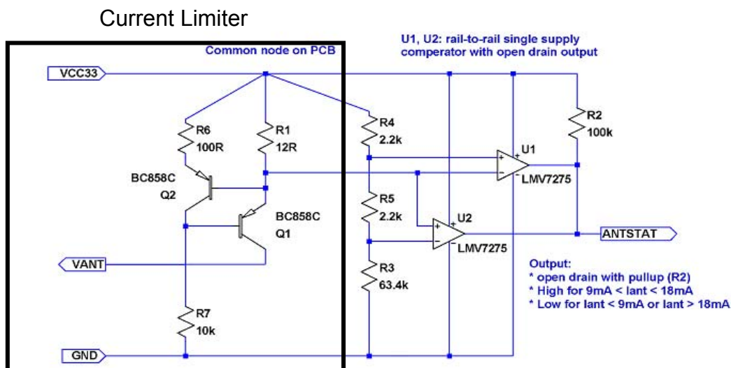
Figure 17: Application note: Antenna sensor adaptation with current limiter
