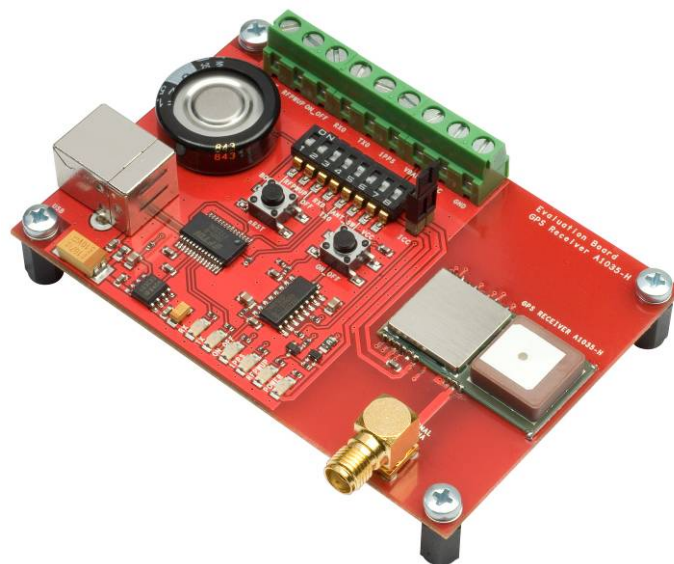
Figure 20: Evaluation kit EVA1035-H
