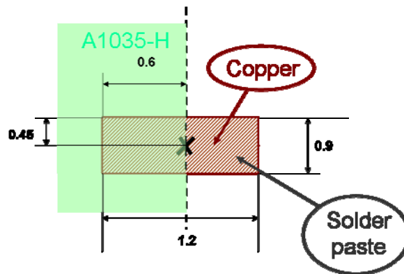
Figure 12: Soldering footprint proposal A1035-H
