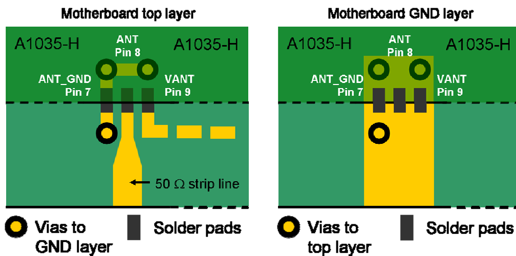
Figure 13: Antenna connector strip line A1035-H
