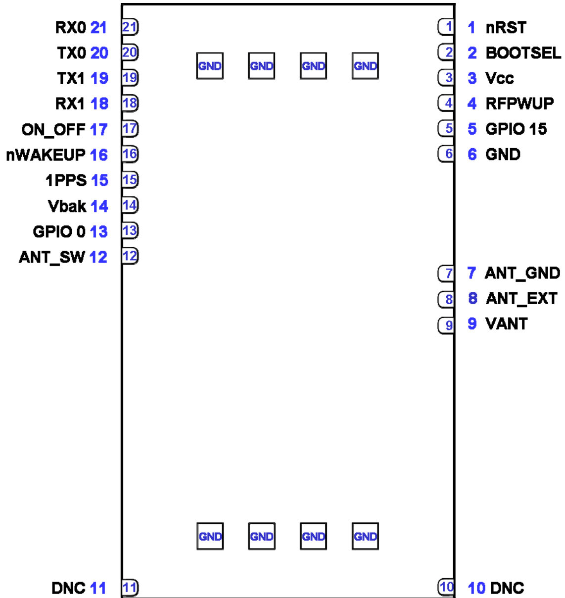
Figure 11: Pin-out information (bottom view) A1035-H
