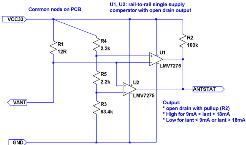
Figure 16: Application note: Antenna sensor adaptation
