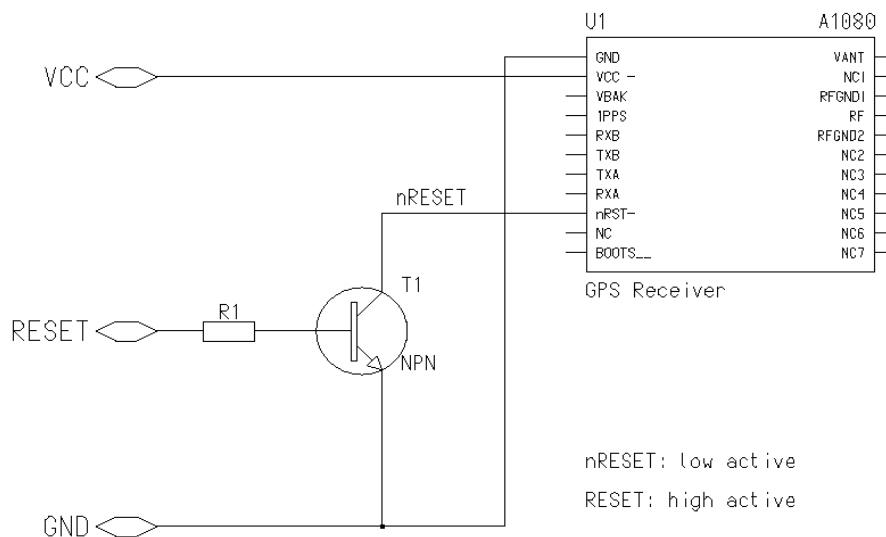
Figure 18: Application note: Recommended external reset circuit
