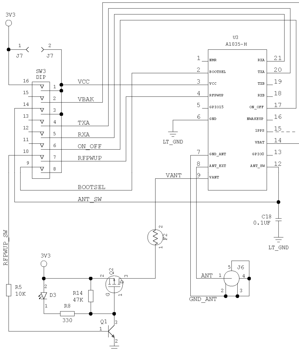
Figure 15: Switching external antenna supply using RFPWUP
