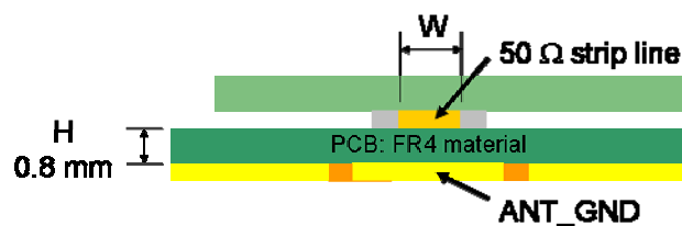
Figure 14: Strip line parameters A1035-H
